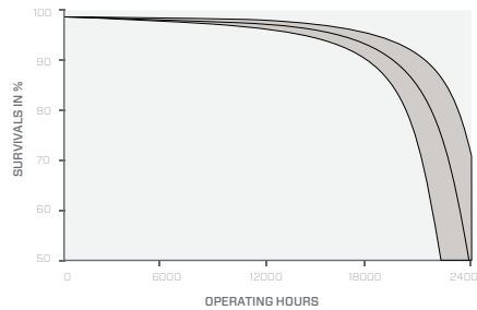
2.1 - LIFE EXPECTANCY
