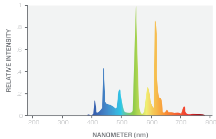
1.1 - SPECTRAL POWER DISTRIBUTION - 4100K (B41)
