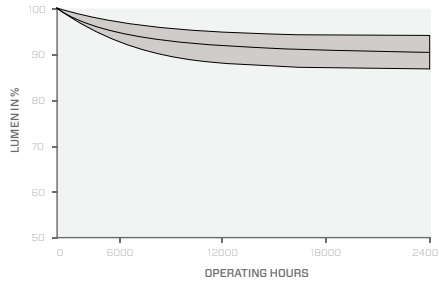
2.2 - LUMEN MAINTENANCE
