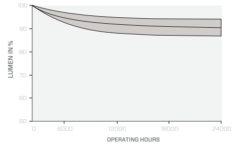
2.2 - LUMEN MAINTENANCE
