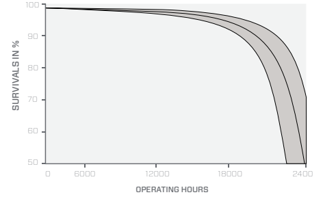
2.1 - LIFE EXPECTANCY
